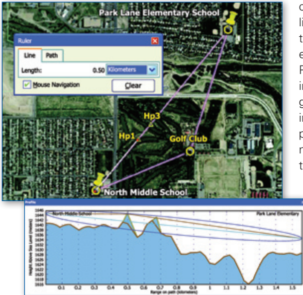
PTP LINKPlanner Google Earth Network View and Path Obstruction Profile
