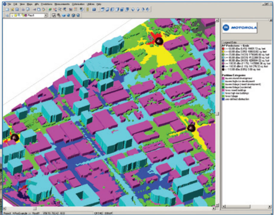
BroadbandPlanner 3D Obstructions and Prediction View
